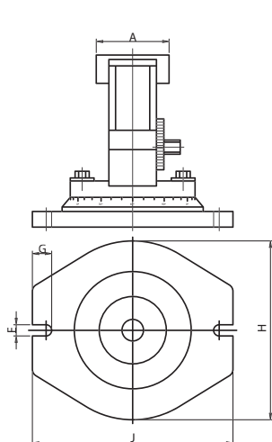
Hydraulic machine vise
